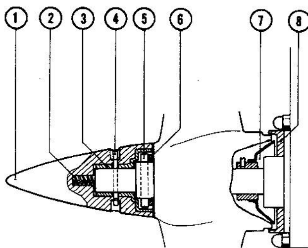
Fig. 3. Propeller with fixed blades
